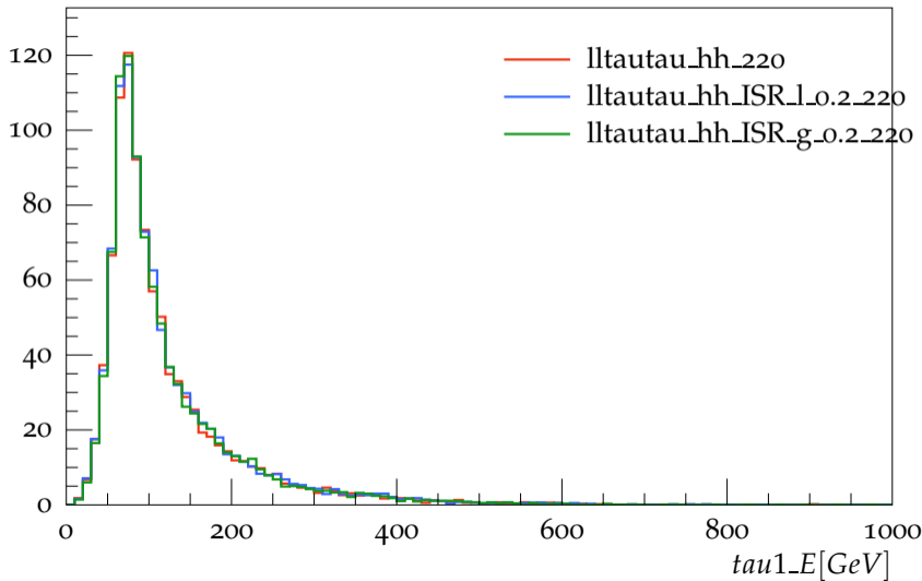
ISR_compare_220GeV_Sample
